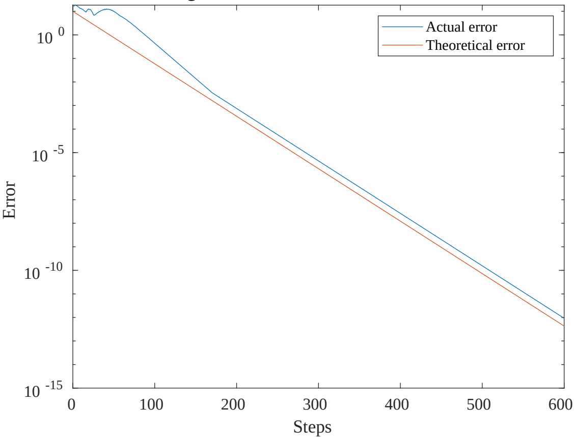
Convergence of the Basic QR Method
